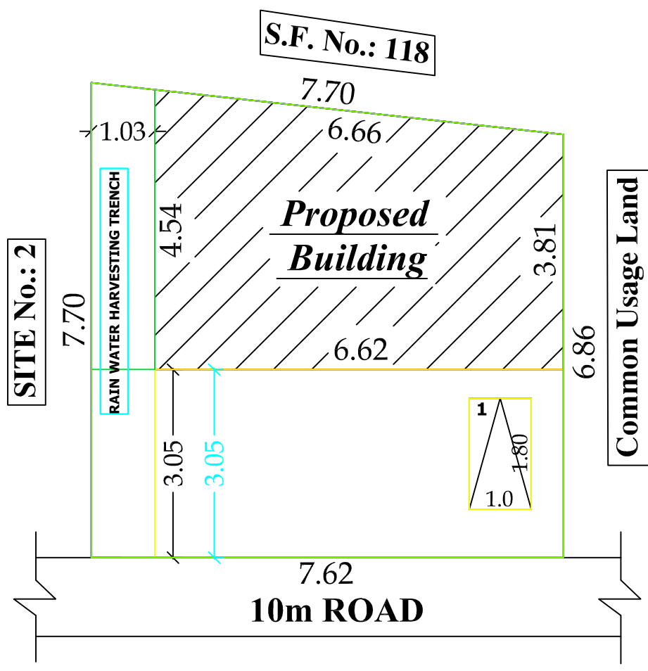
SITE PLAN
