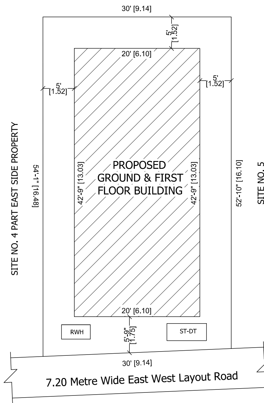
SITE PLAN
