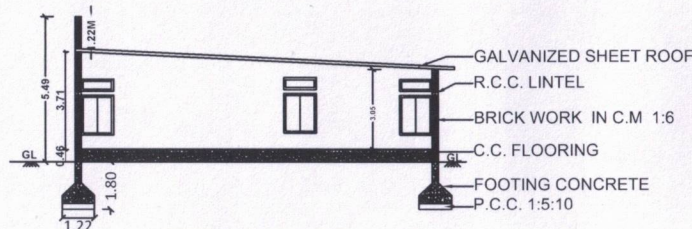
SECTION AT AA
