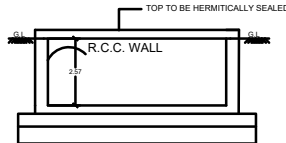
RWH SECTION (SAMPLE)
