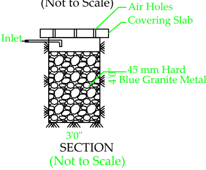
Rain Water Percolation Pit (Not to Scale)
