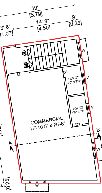
TYPICAL GROUND & FIRST FLOOR PLAN
