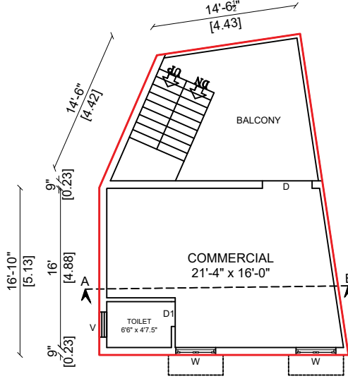
TYPICAL GROUND & FIRST FLOOR PLAN
