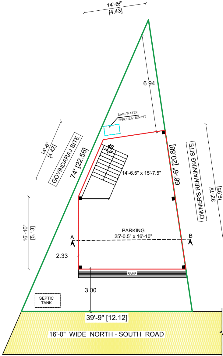
SITE CUM STILT FLOOR PLAN
