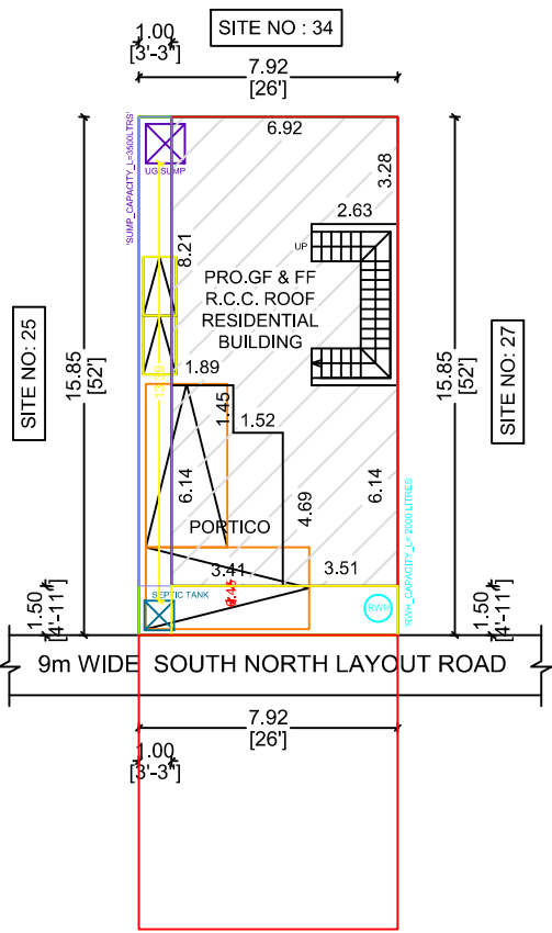
SITE PLAN
