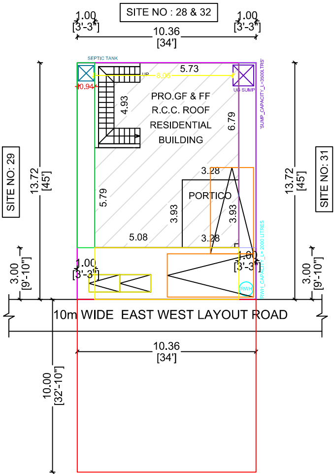
SITE PLAN
