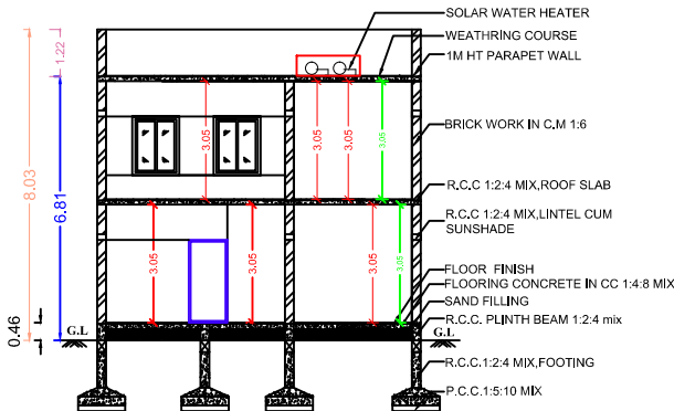
SECTION AT ( B - B )
