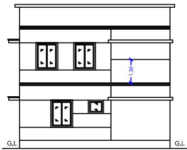
FRONT ELEVATION AT - A
