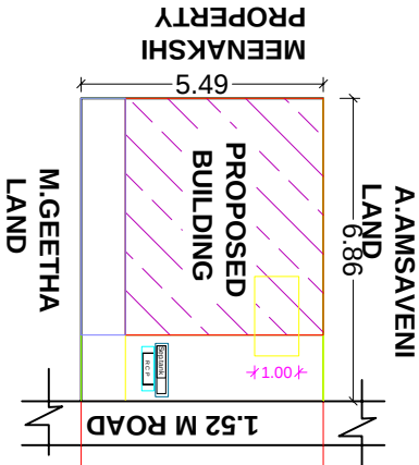
SITE PLAN
