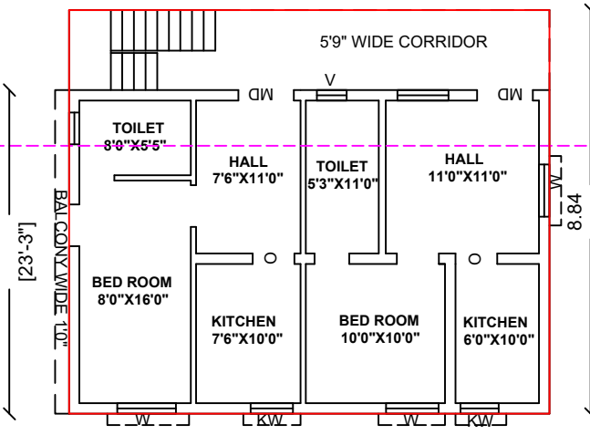
PRO.FIRST FLOOR
