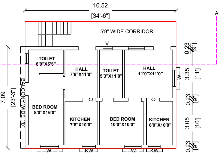
PRO.SECOND FLOOR
