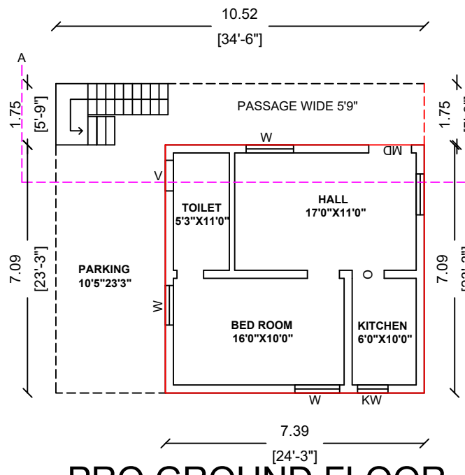
PRO.GROUND FLOOR
