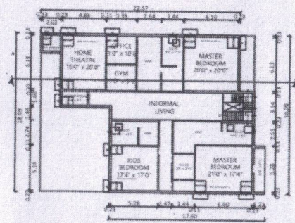
PRO. FIRST FLOOR PLAN
