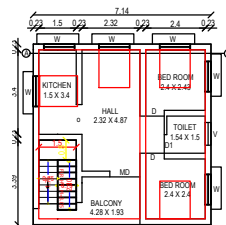
PROPOSED ADDITIONAL FIRST FLOOR BUILDING
