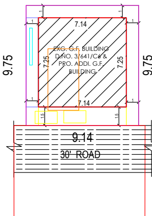
SITE PLAN
