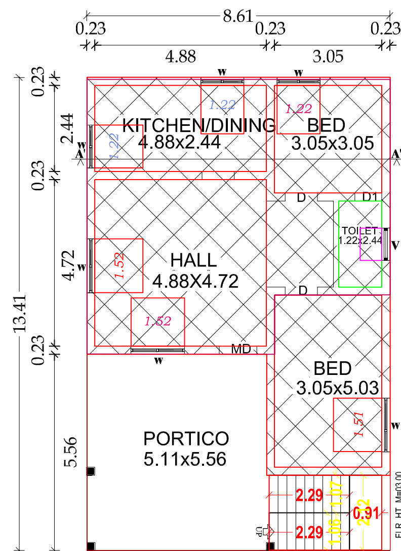
EXG. AND PRO. ADD. GROUND FLOOR PLAN
