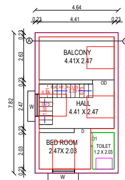
PROPOSED FIRST FLOOR BUILDING
