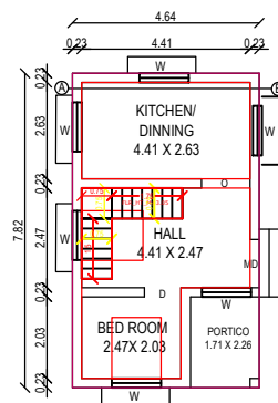
PROPOSED GROUND FLOOR BUILDING
