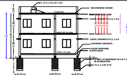
SECTION
