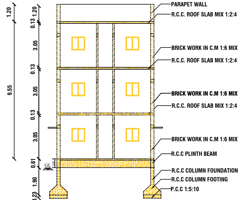
CROSS SECTION AT A-A
