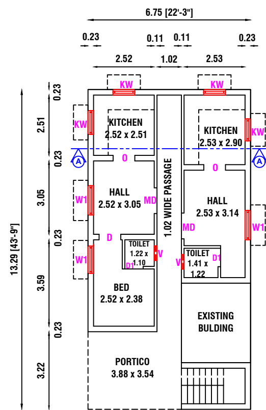
EXISTING GROUND AND ADD.PROPOSED GROUND FLOOR PLAN
