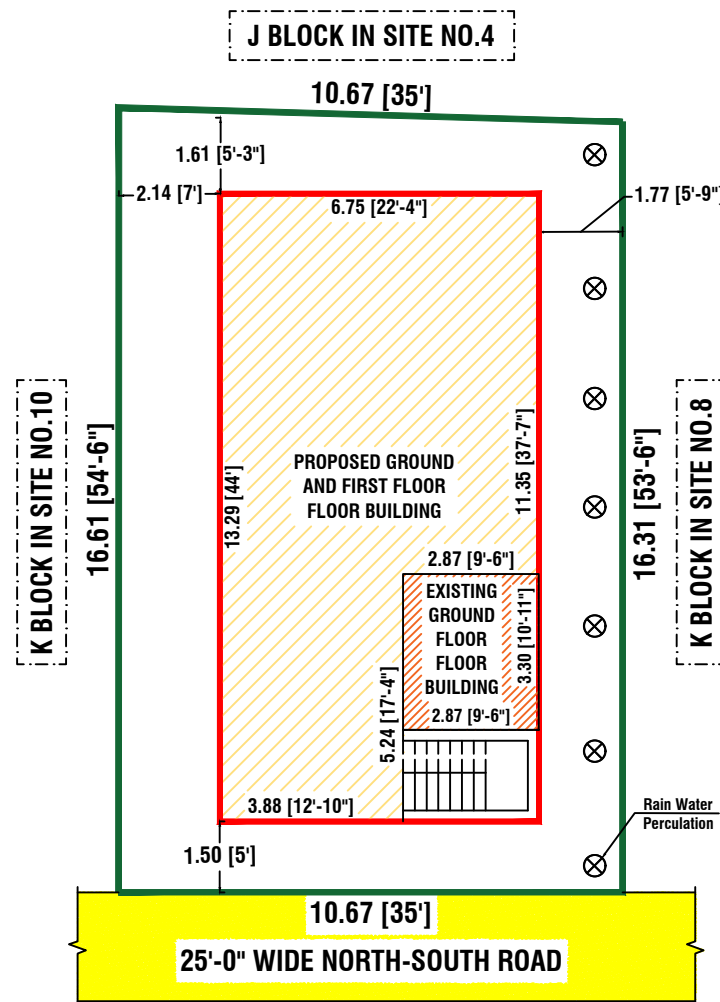
SITE PLAN
