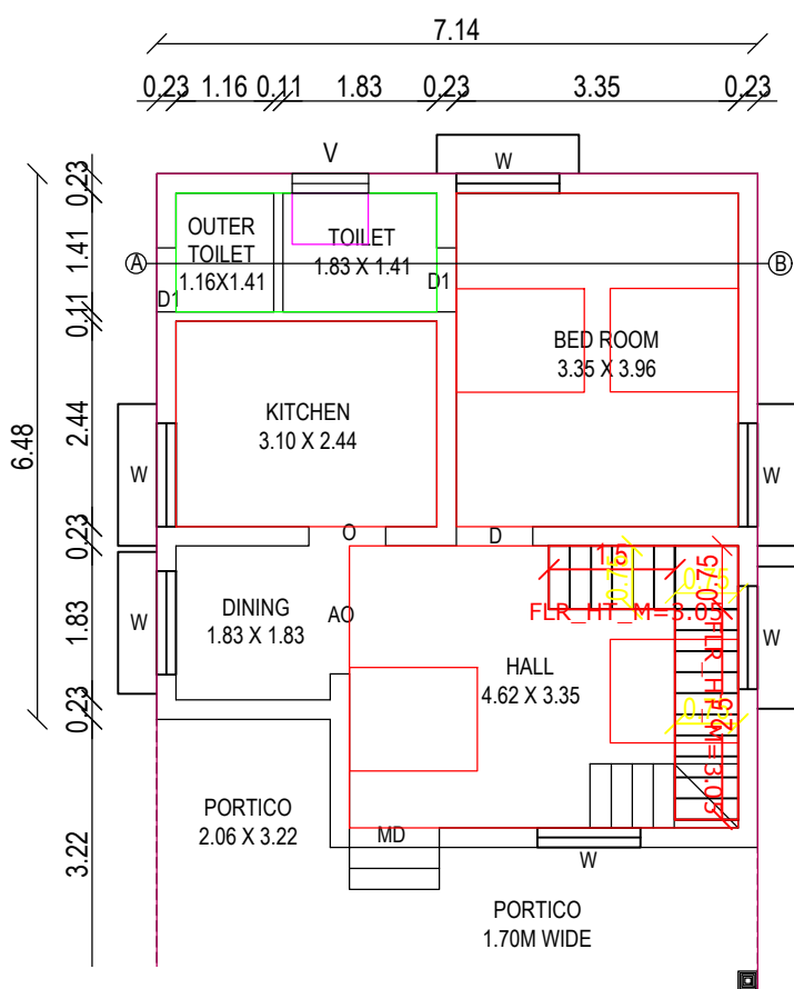
PROPOSED GROUND FLOOR BUILDING
