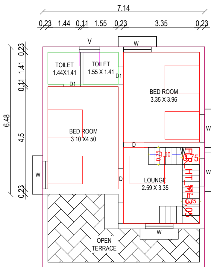
PROPOSED FIRST FLOOR BUILDING
