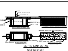
SEPTIC TANK DETAIL
