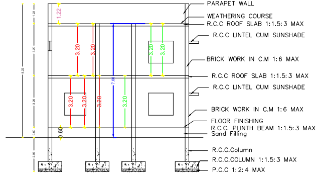
SECTION
