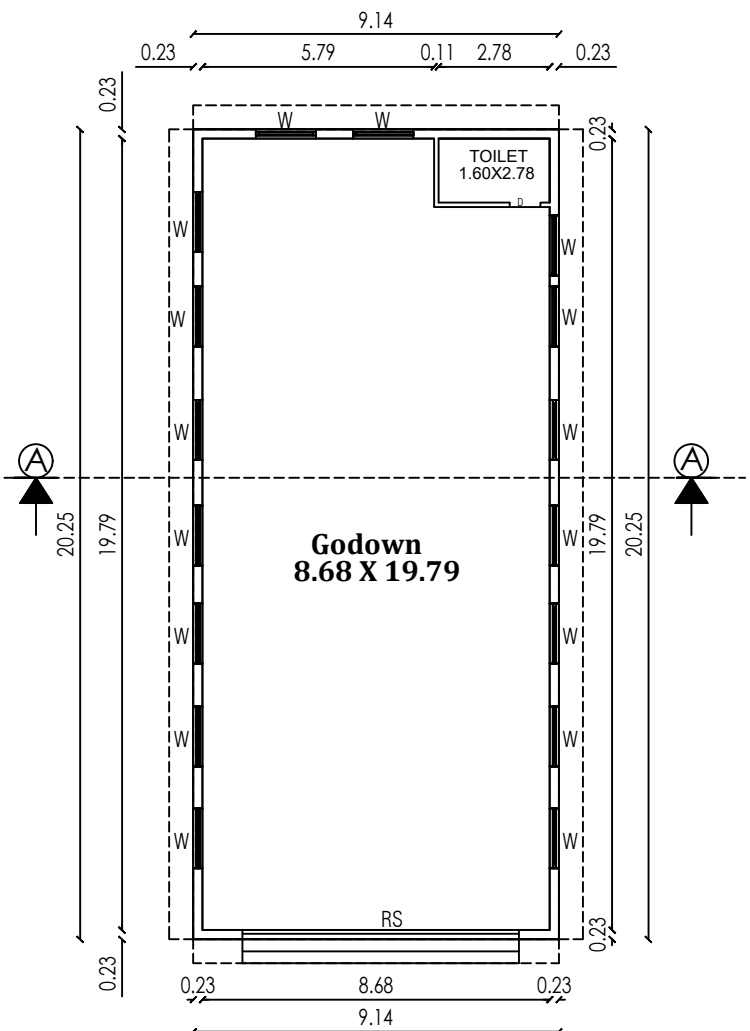
PLAN
