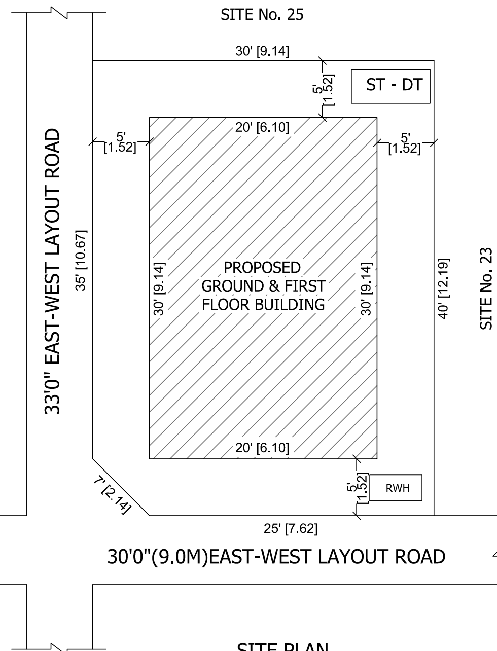
SITE PLAN
