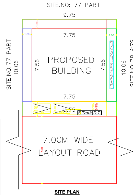
SITE PLAN
