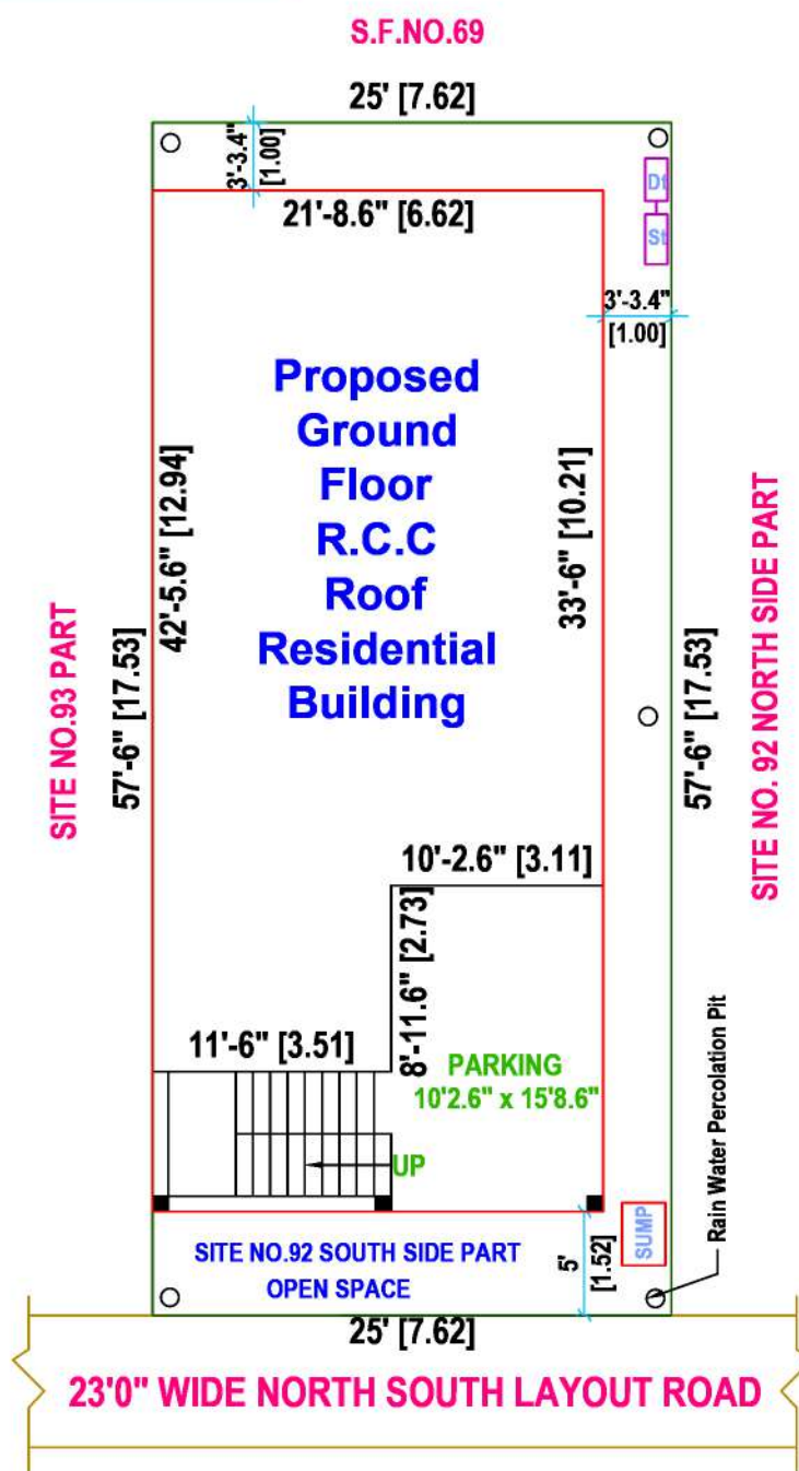
SITE PLAN (SCALE - 1" : 8' 0")
