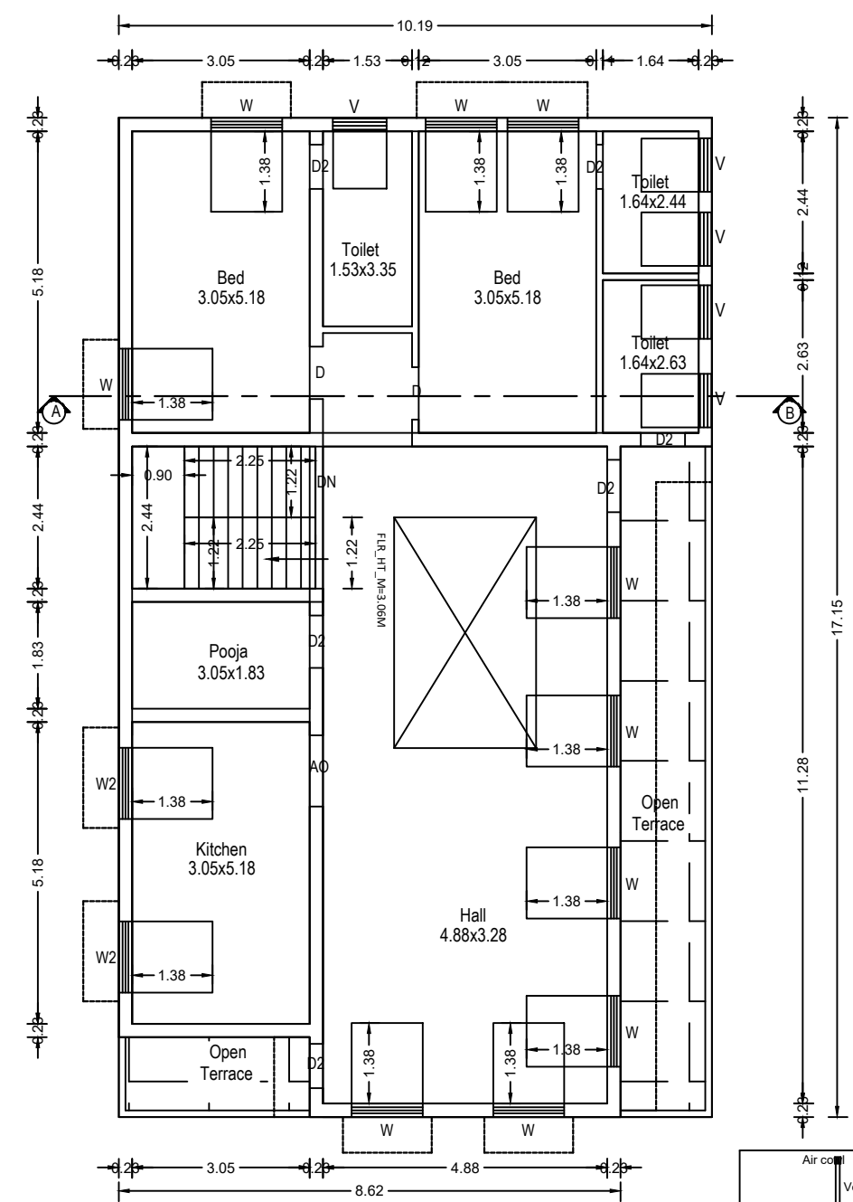
Plan Scale 1:100 Pro. First floor
