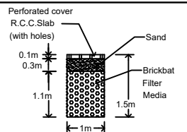
STING SECTION
