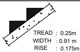
STAIRCASE DETAIL:
