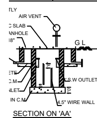
SECTION ON 'AA'
