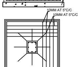
FOOTING DETAIL (SCALE: NTS)
