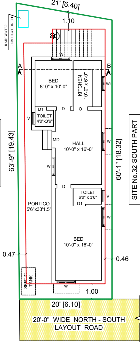
SITE CUM GROUND FLOOR PLAN
