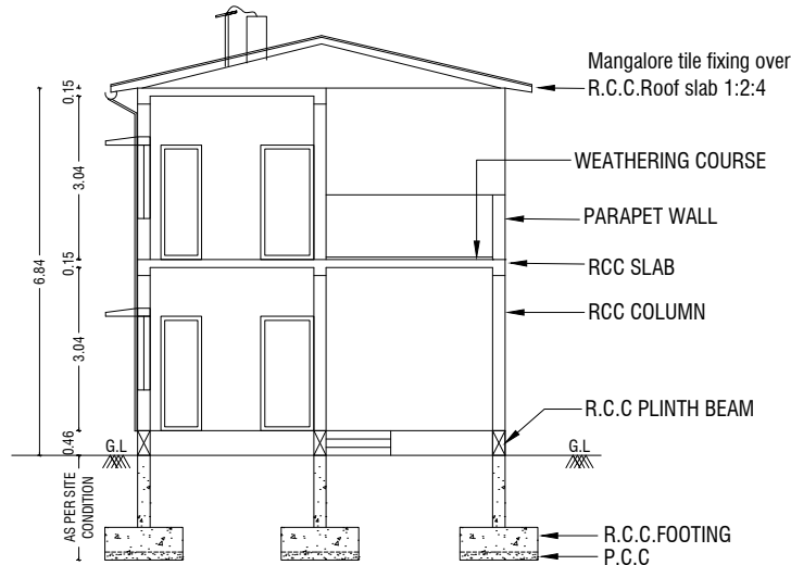
SECTION ON "AA" @ NORTH SIDE
