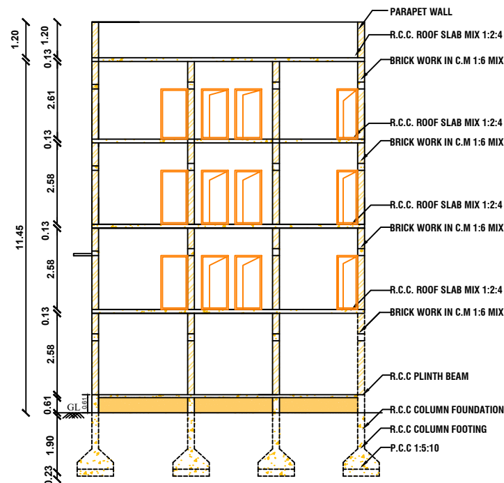
CROSS SECTION AT A-A
