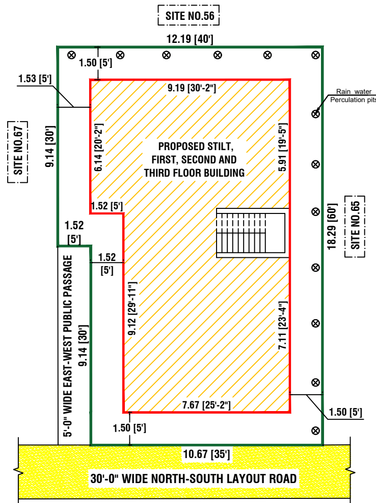
SITE PLAN
