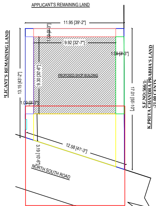
SUPER IMPOSED PLAN TAKEN FOR CONSTRUCTION)
