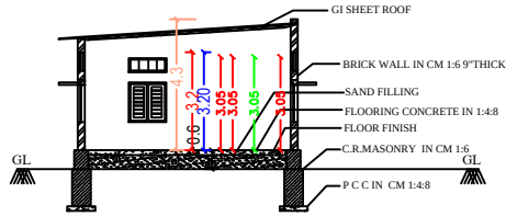
CROSS SECTION
