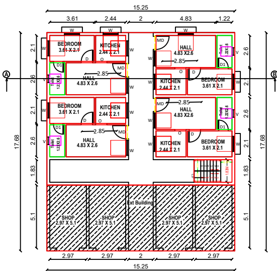
PRC GROUND FLOOR PLAN
