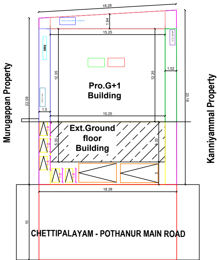
SITE PLAN (SCALE 1" : 8' 0")
