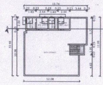
PROPOSED SECOND FLOOR
