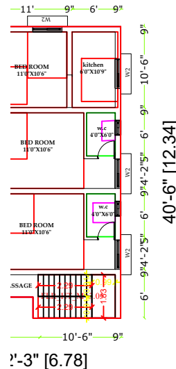
PROPOSED FIRST FLOOR PLAN
