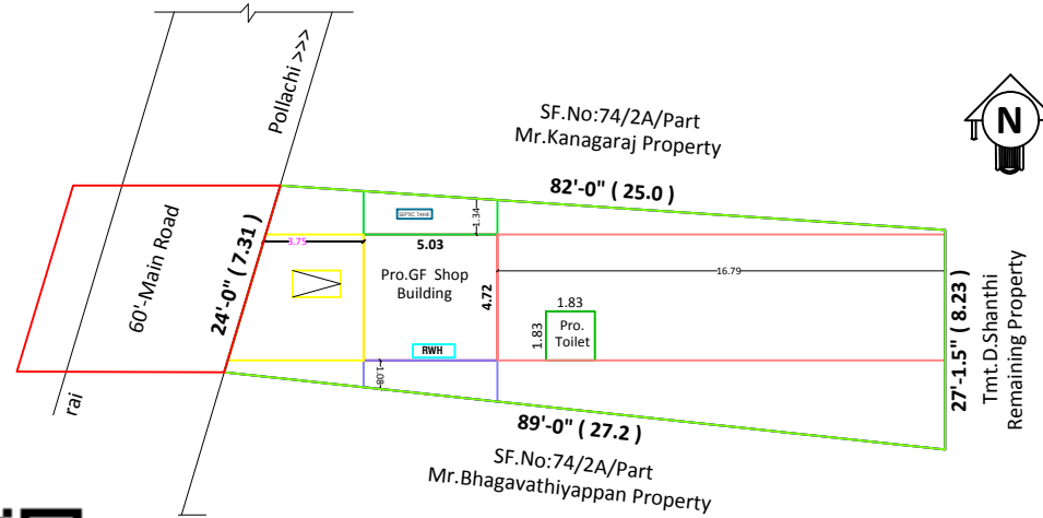
SITE PLAN
