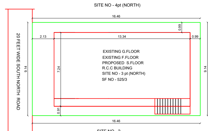
SITE PLAN
