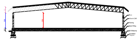
SECTION ON "AA"
