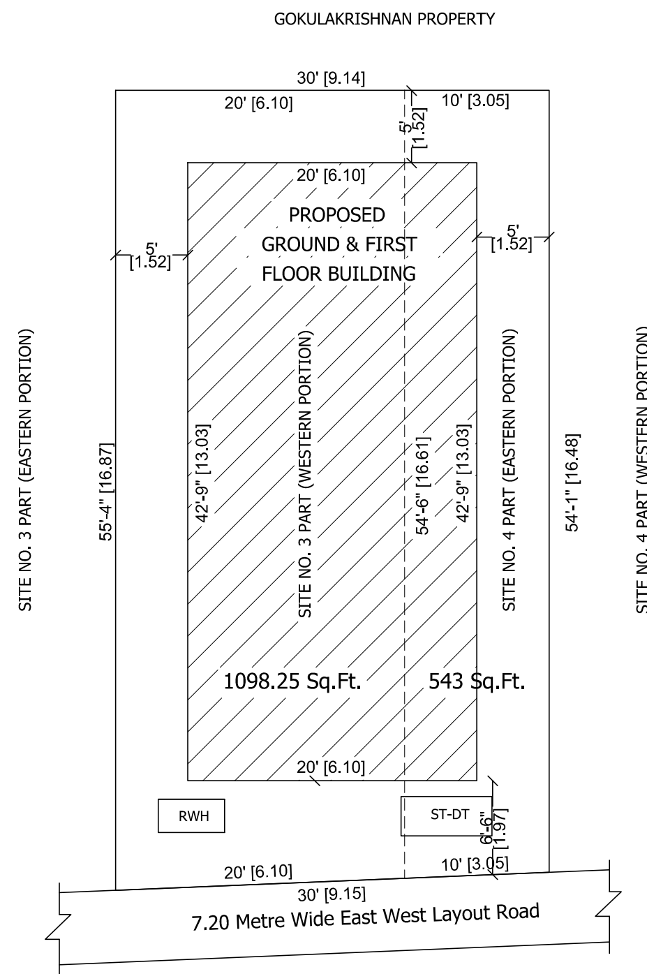
SITE PLAN
