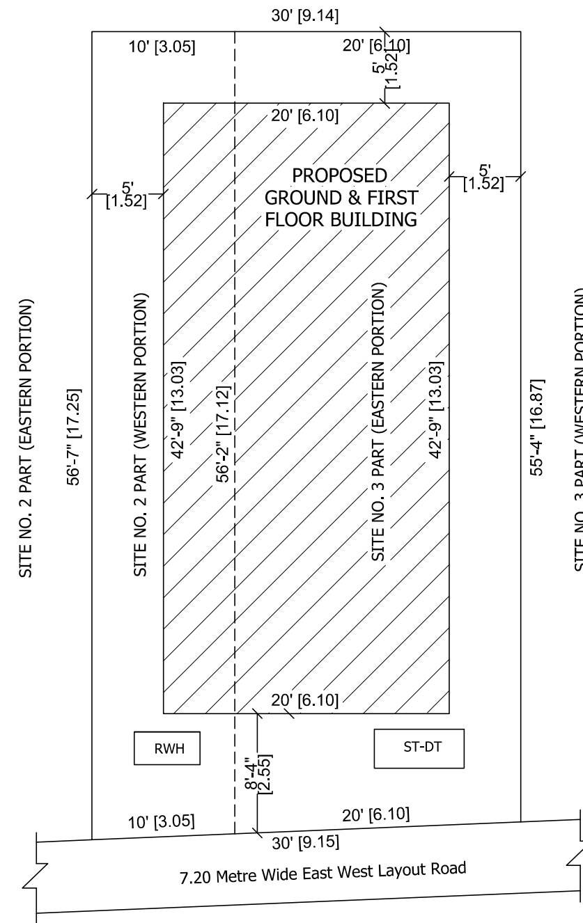
SITE PLAN
