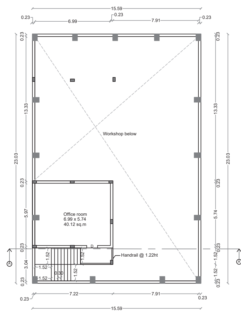
MEZZANINE FLOOR PLAN
