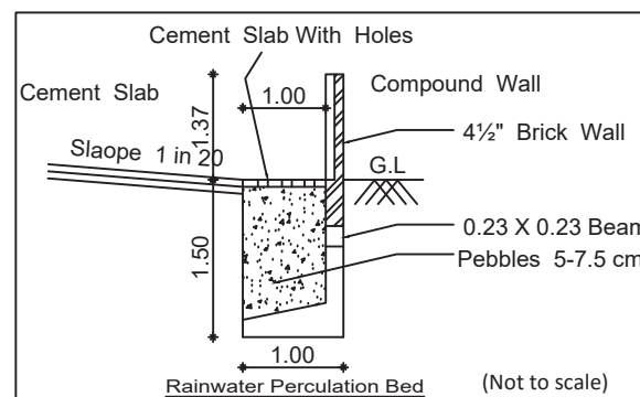
Cement Slab With Holes (Not to scale)
