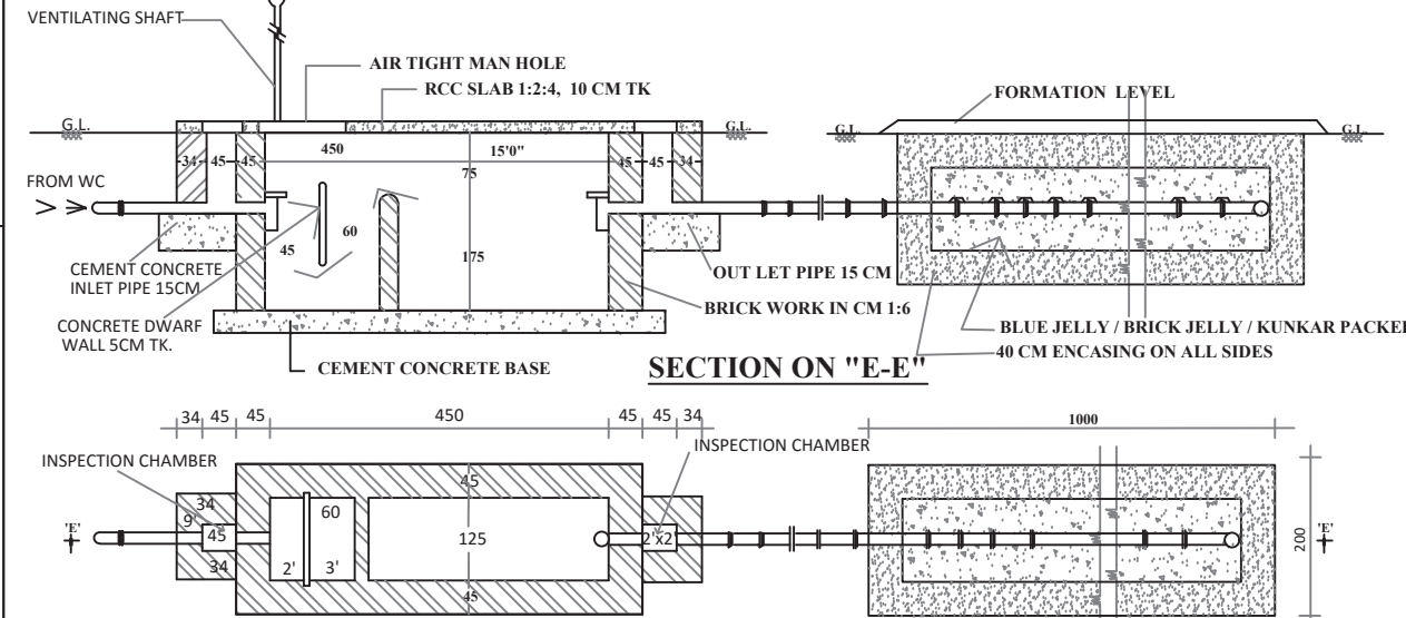
SEPTIC TANK
