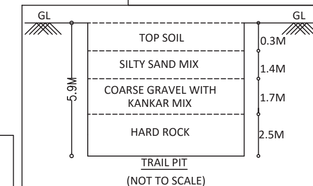
TRAIL PIT (NOT TO SCALE)
