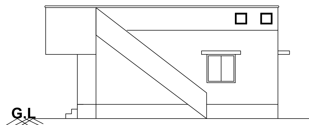
FRONT ELEVATION
