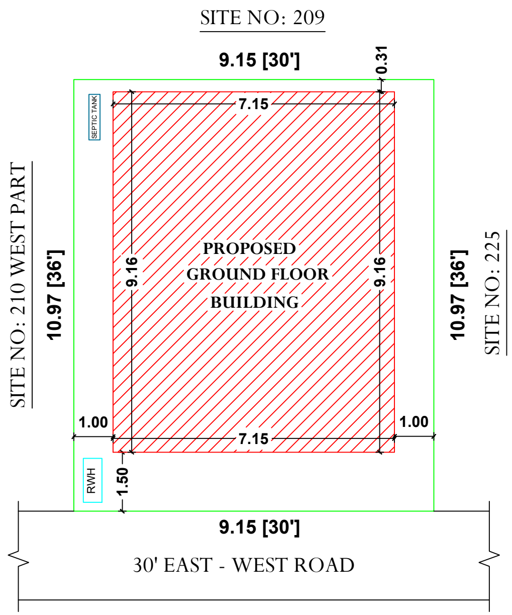
SITE PLAN
