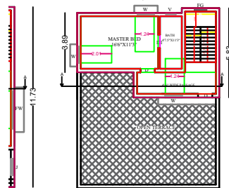
PLAN PROPOSED FIRST FLOOR PLAN
