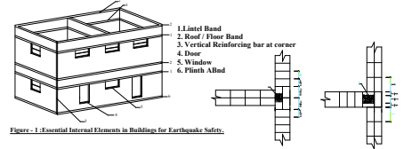
Figure - 1: Essential Elements for Earthquake Safety.
