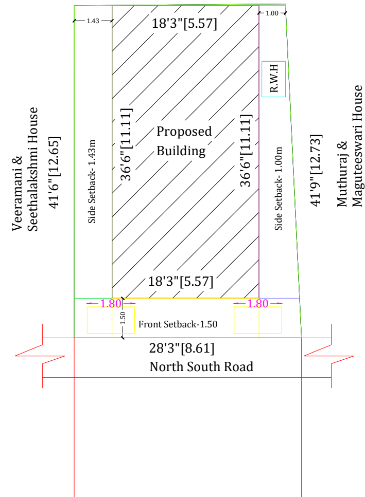
SITE PLAN
