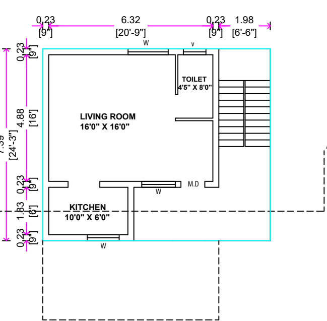
PROPOSED SECOND FLOOR
