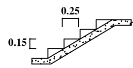
STAIR CASE DETAILS: (Not to Scale)
