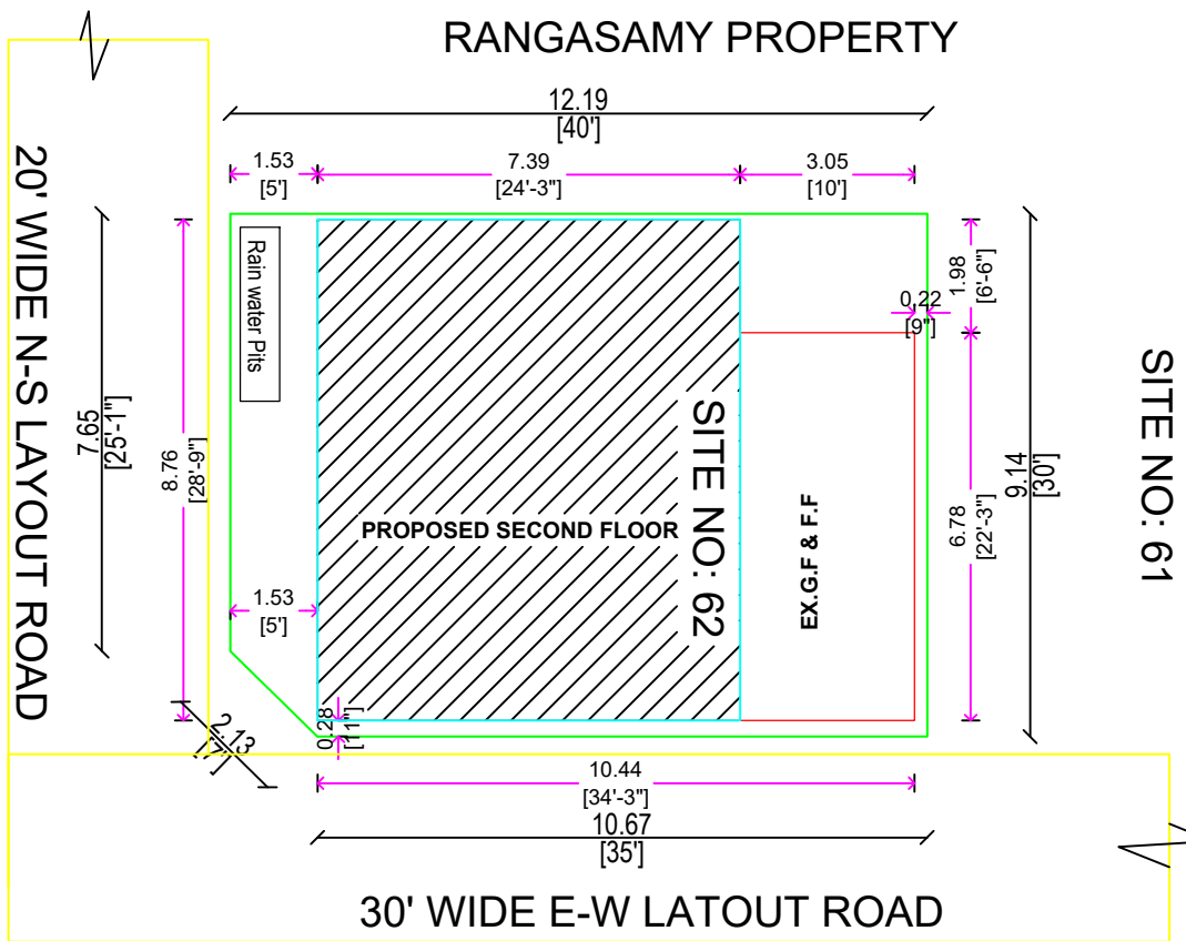
SITE PLAN
