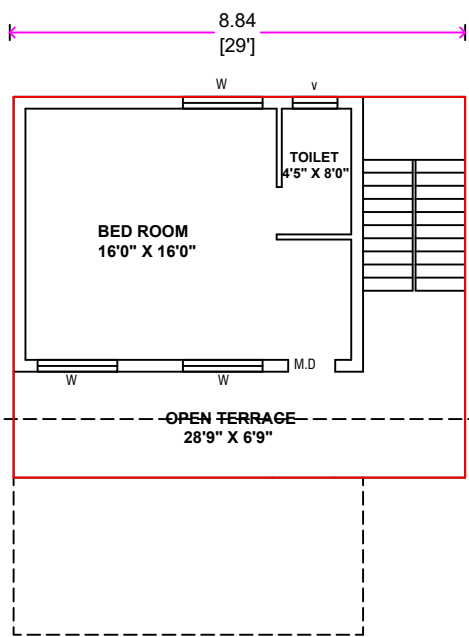
EXISITING FIRST FLOOR
