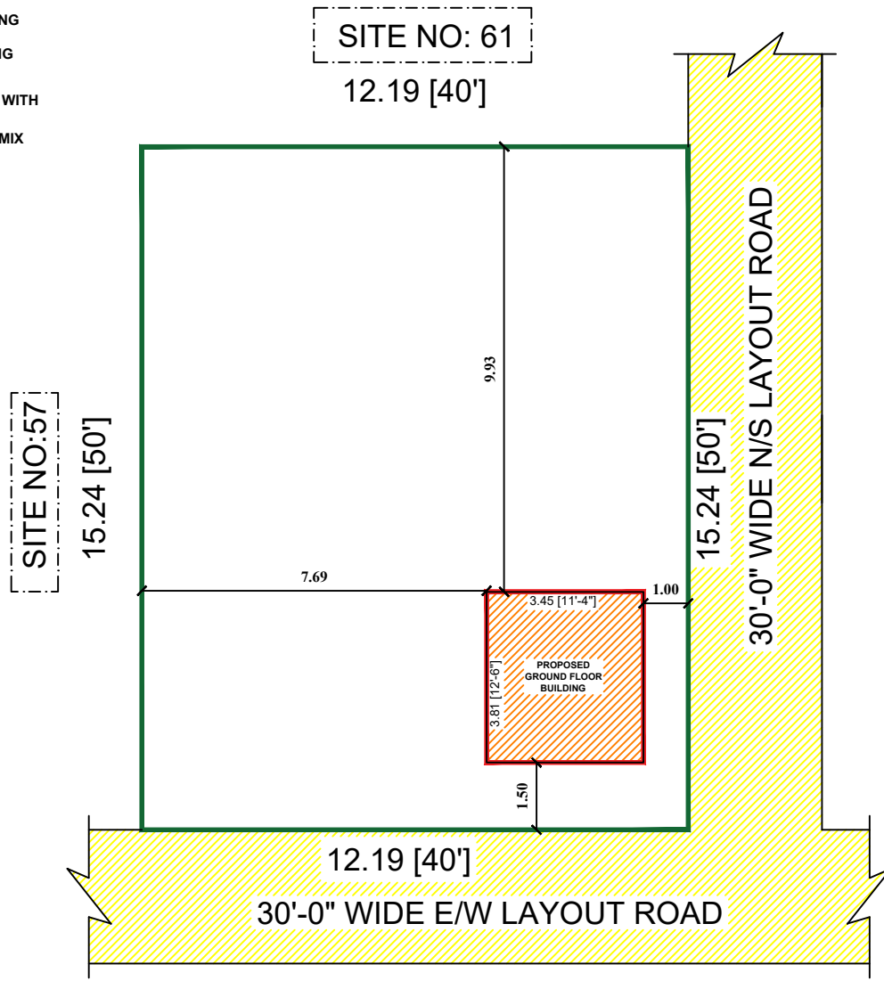
SITE PLAN
