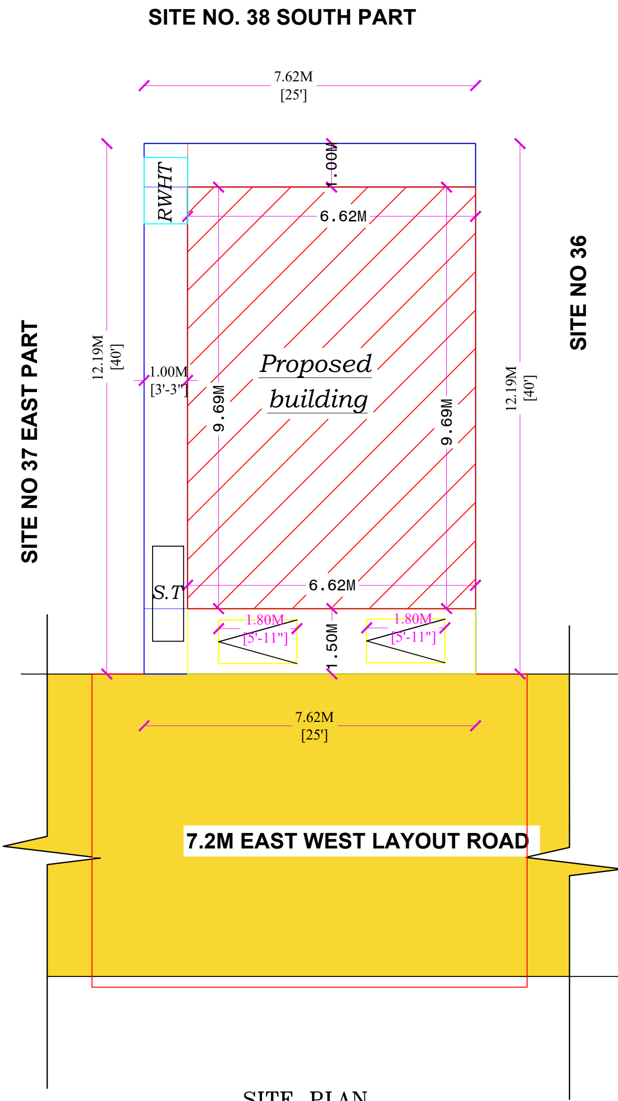
SITE PLAN
