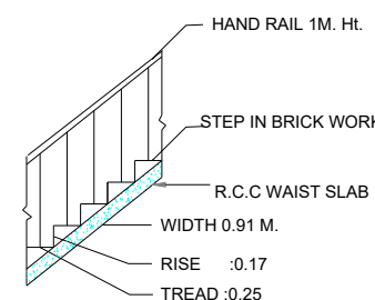
STAIR DETAIL
