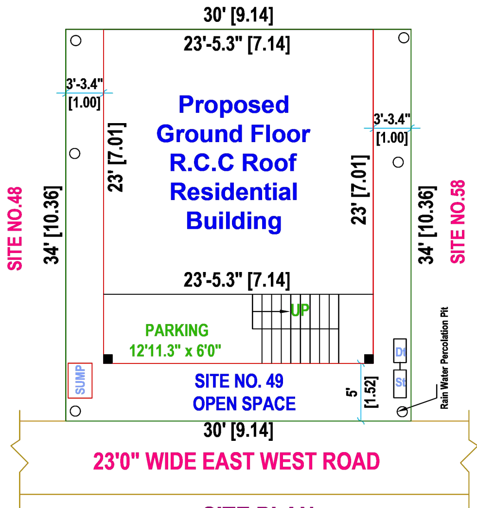
SITE PLAN (SCALE - 1" : 8' 0")
