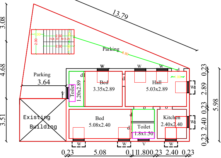
PLAN for Existing & Proposed Ground Floor
