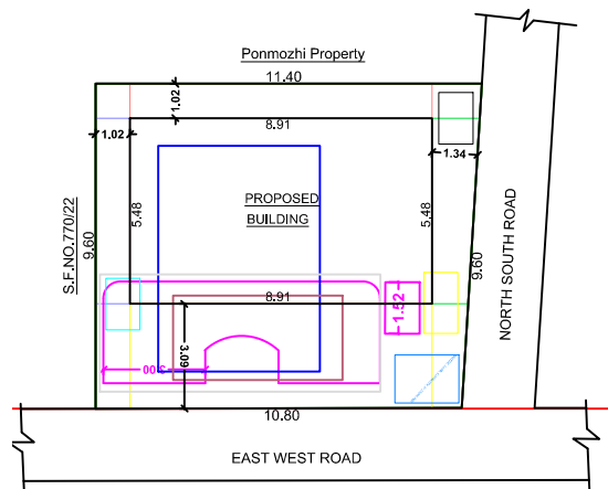
SITE PLAN
